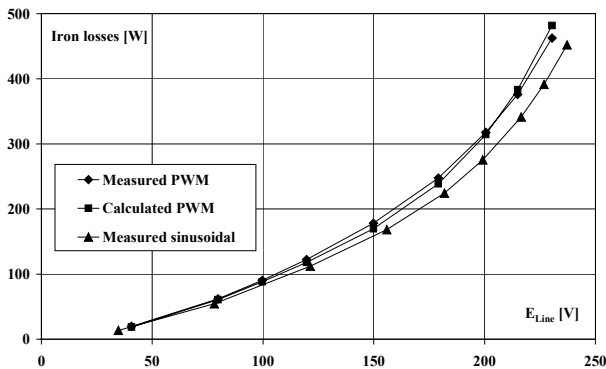
Fig. 12: Predicted and measured iron losses with PWM supply (fundamental frequency = 50 Hz, switching frequency = 2 kHz, variable DC bus voltage).
