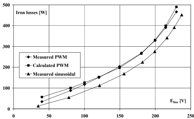
Fig. 11: Predicted and measured iron losses with PWM supply (fundamental frequency = 50 Hz, switching frequency = 2 kHz, variable modulation index)
