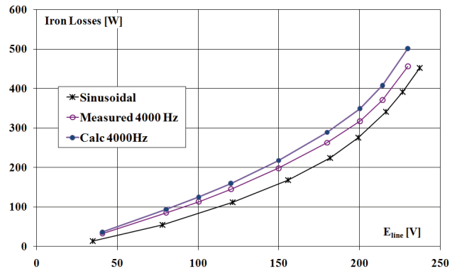
Fig.13: Predicted and measured iron losses with PWM supply (fundamental frequency = 50 Hz, switching frequency = 4 kHz, variable modulation index)
