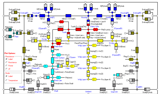
Fig.1: Lumped Circuit for an induction motor thermal model
